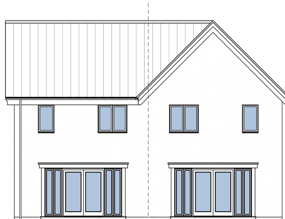
REAR ELEVATION
