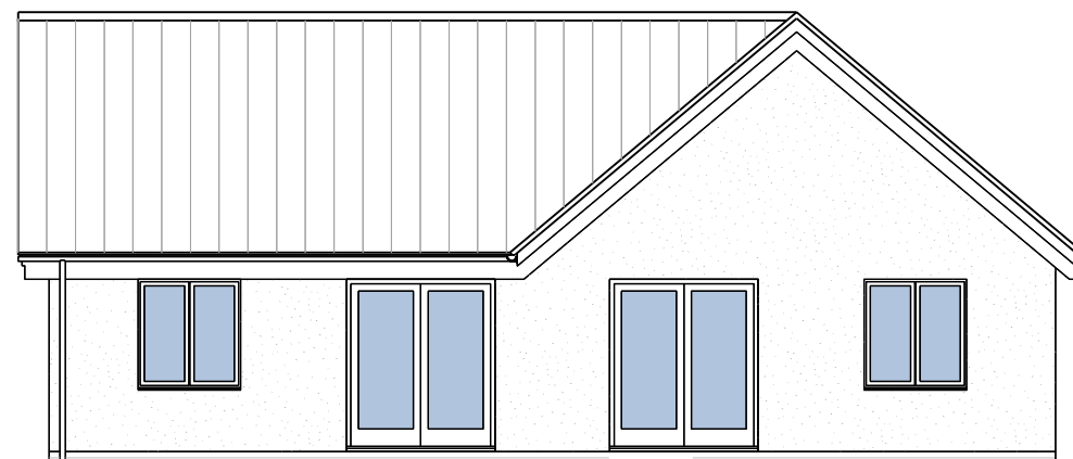
REAR ELEVATION - SEMI DETACHED
