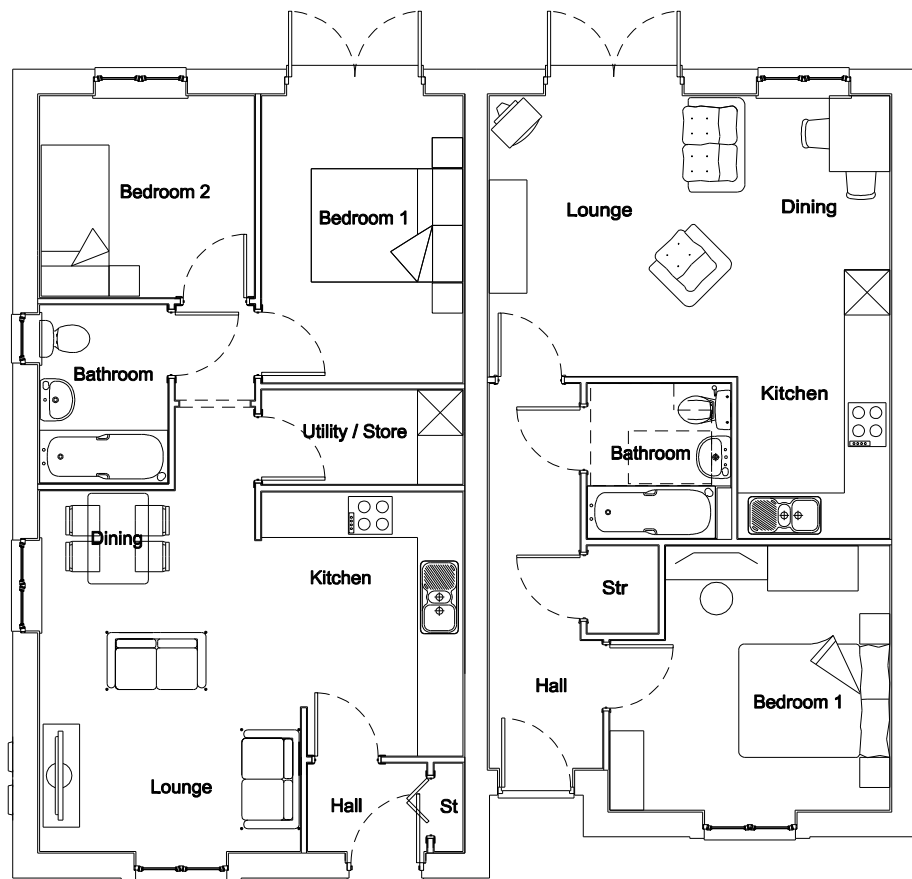
Eastbourne GROUND FLOOR PLAN
