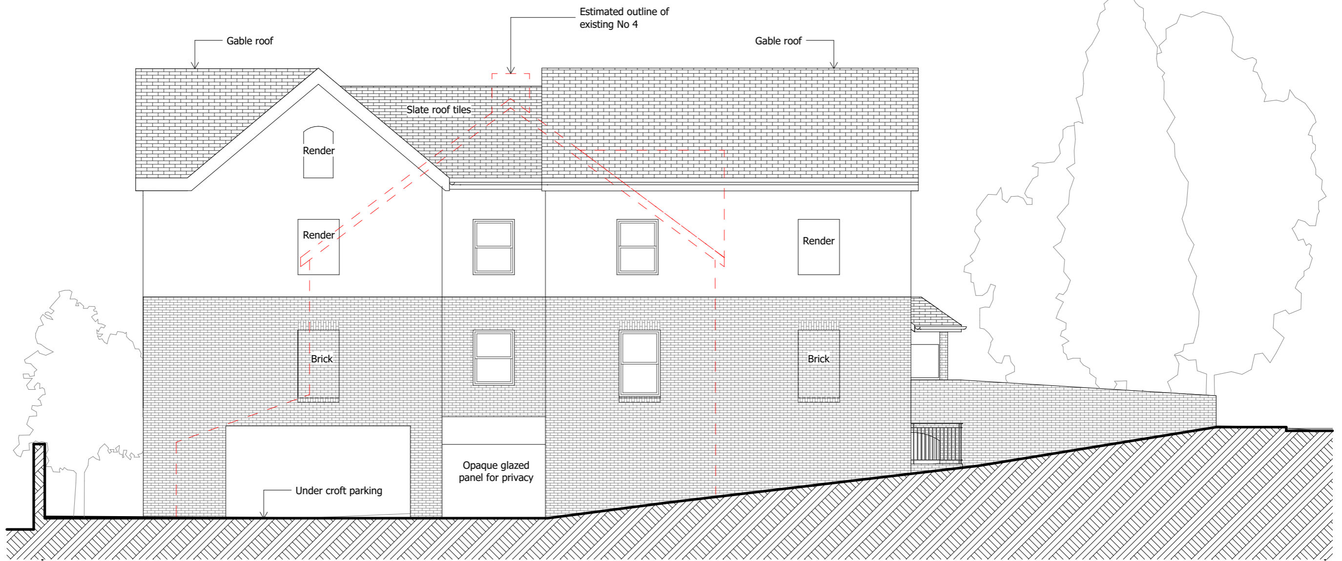
West Elevation
