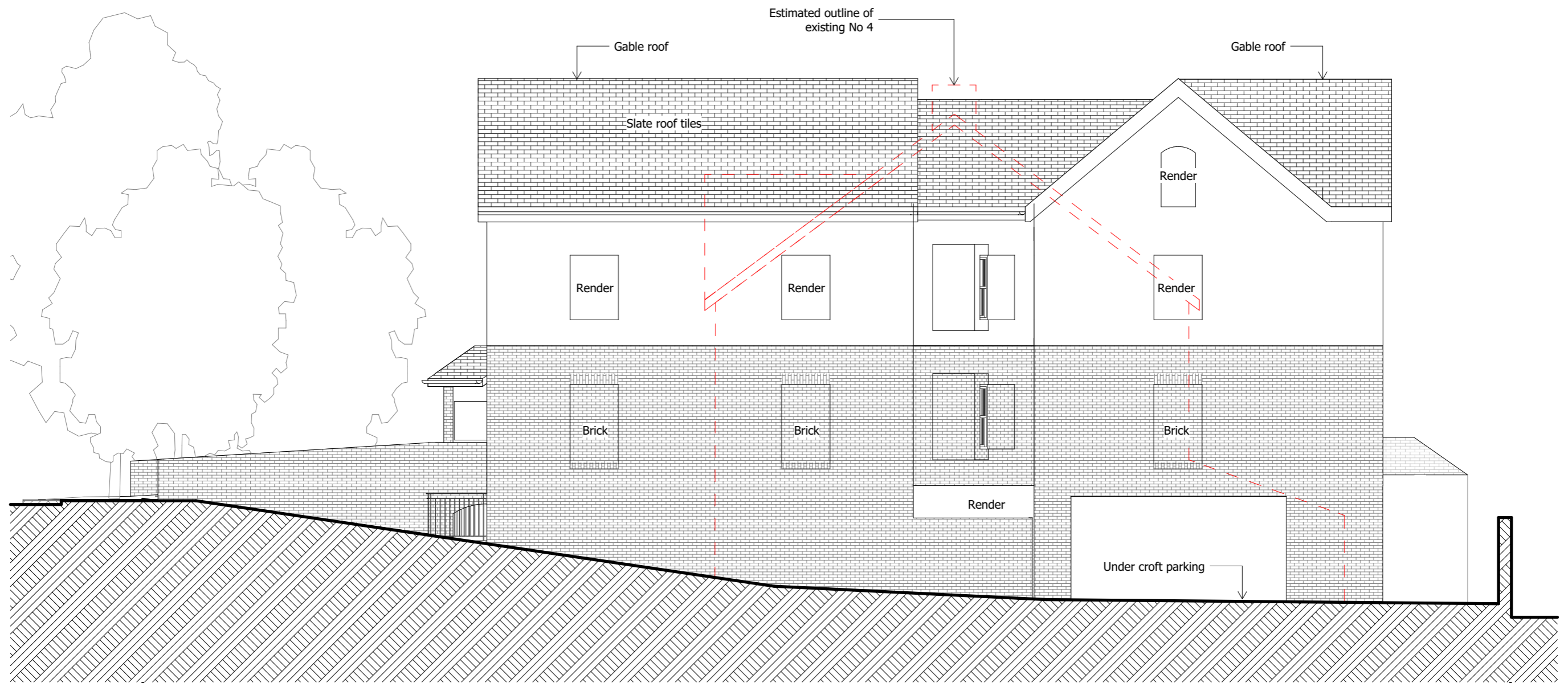
East Elevation
