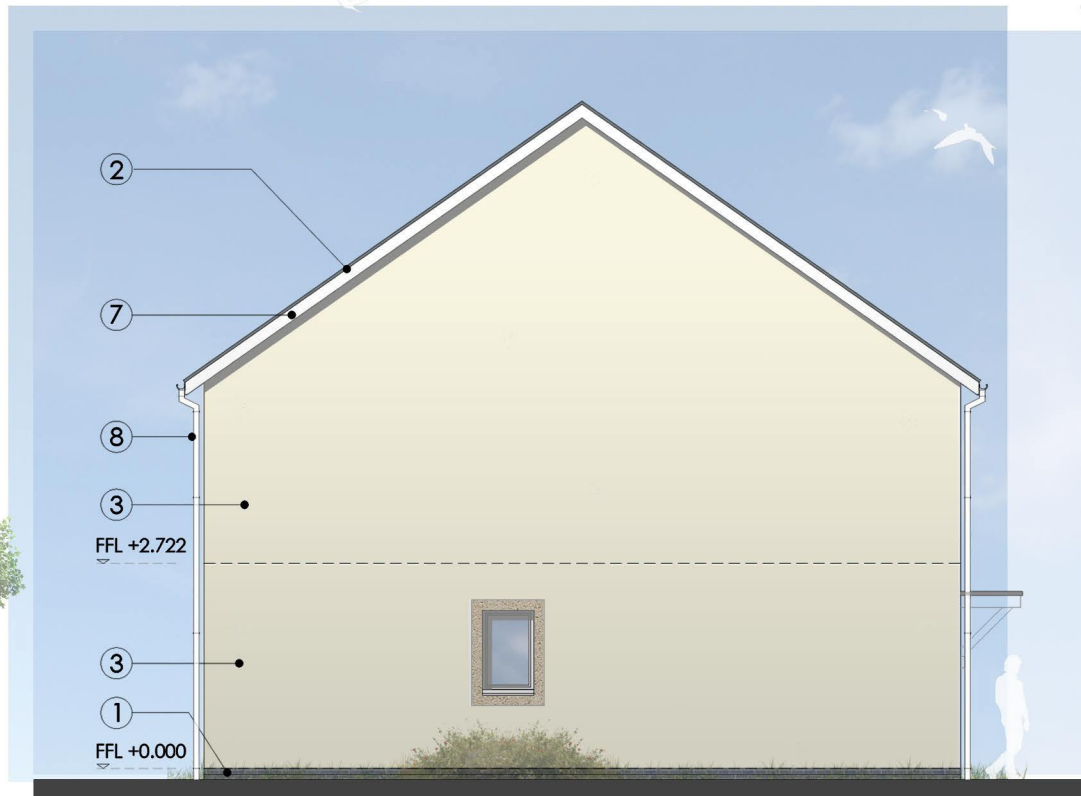
LEFT SIDE ELEVATION OPTION 2
