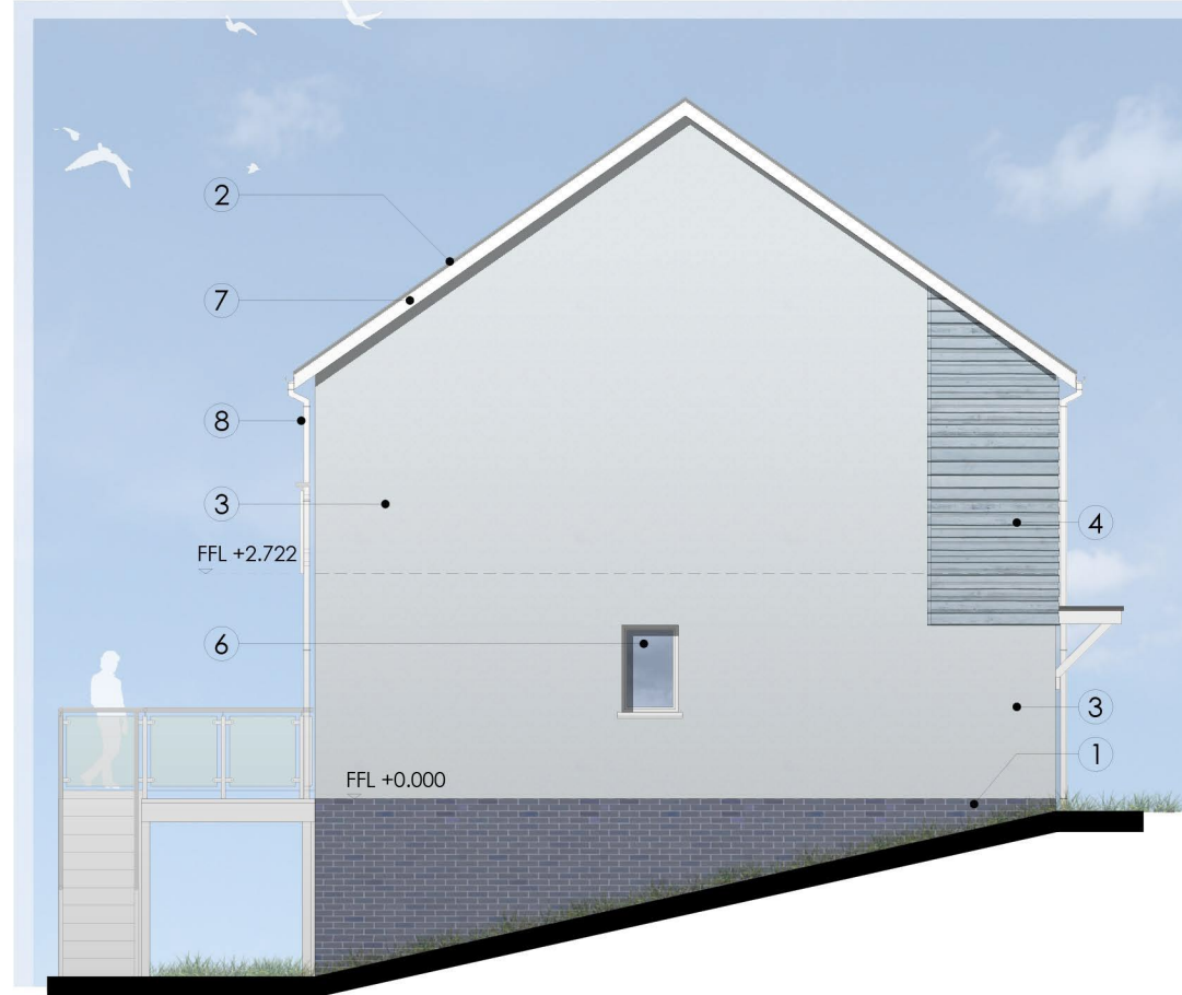
LEFT SIDE ELEVATION OPTION 6
