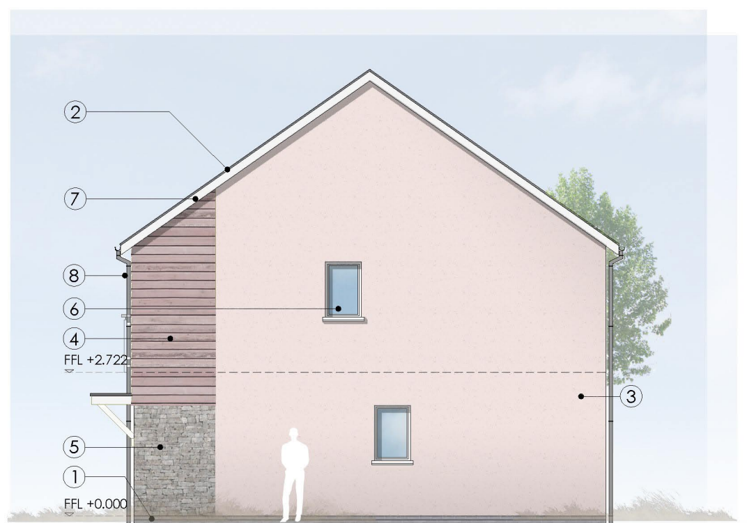
RIGHT SIDE ELEVATION OPTION 6
