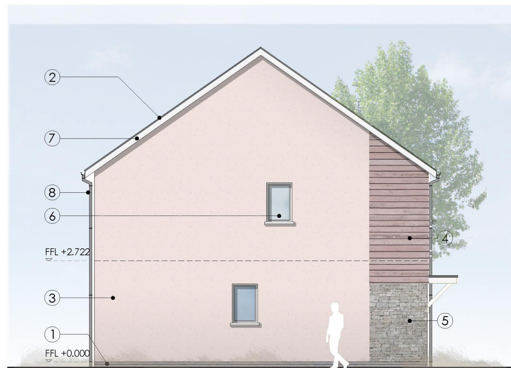
LEFT SIDE ELEVATION OPTION 6
