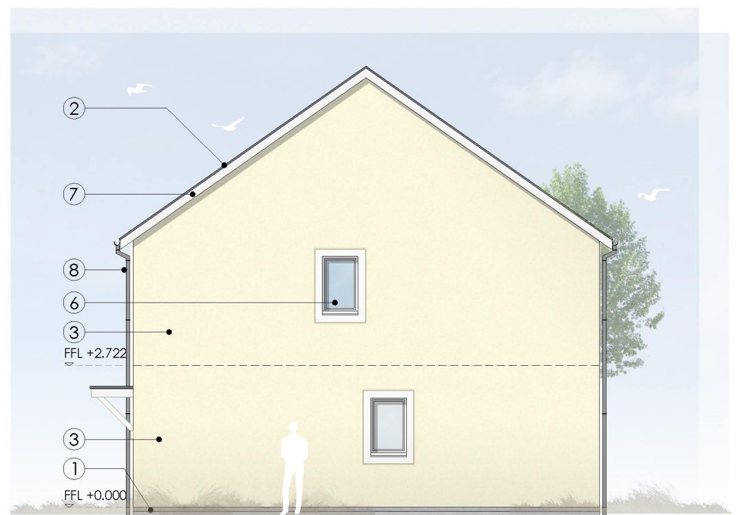
RIGHT SIDE ELEVATION OPTION 4
