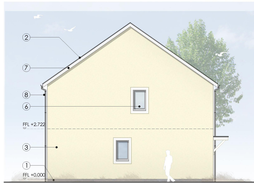
LEFT SIDE ELEVATION OPTION 4
