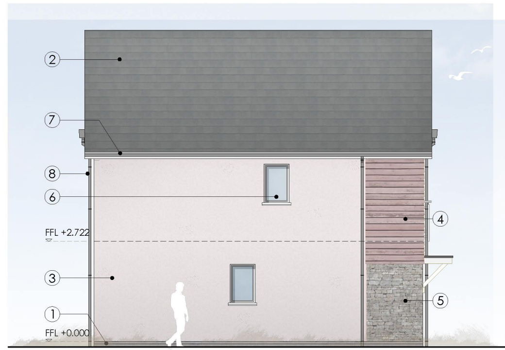
LEFT SIDE ELEVATION OPTION 2
