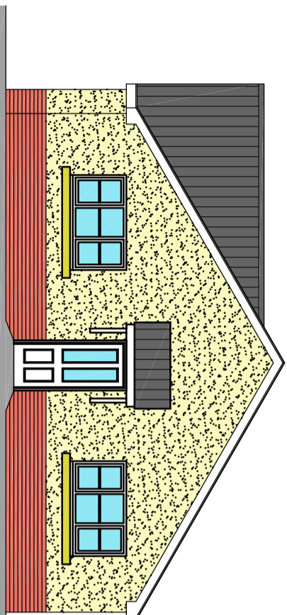
ENTRANCE ELEVATION
